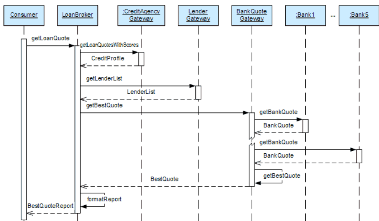
Loan Broker Sequence Diagram
