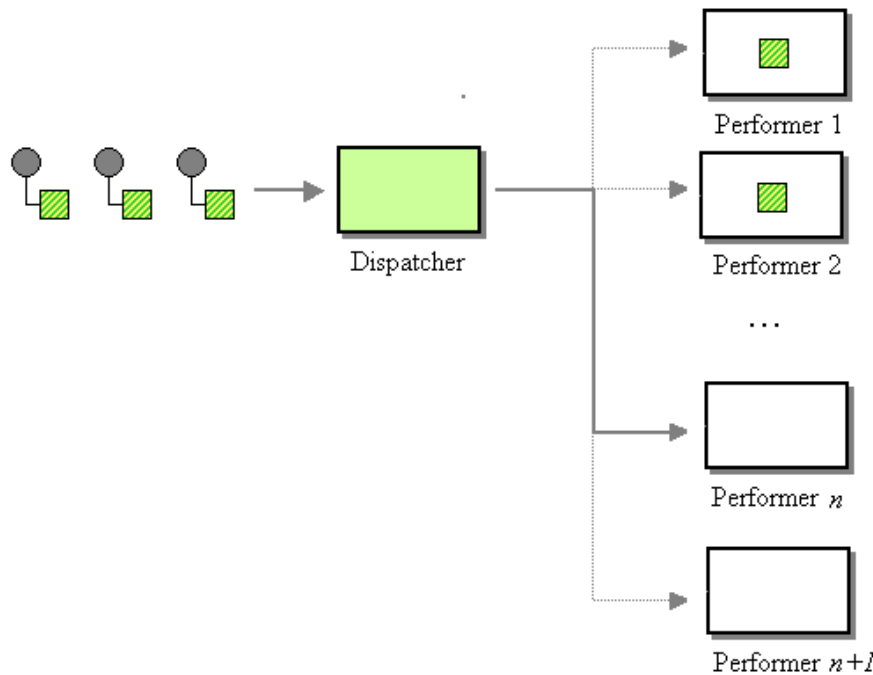
The Message Dispatcher in context
