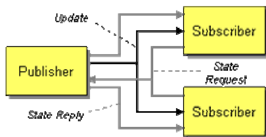
Publish/Subscribe using the Pull Model
