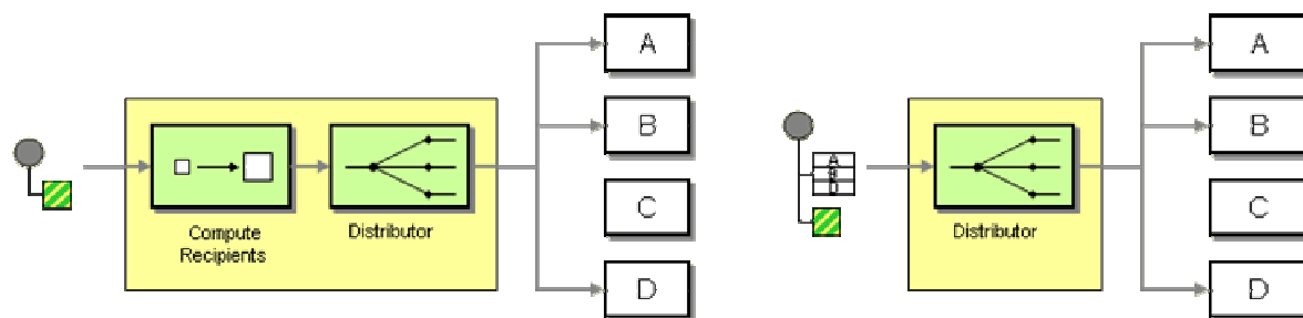
A Recipient List Can Compute the Recipients (left) or Have Another Component Provide A List (right)
